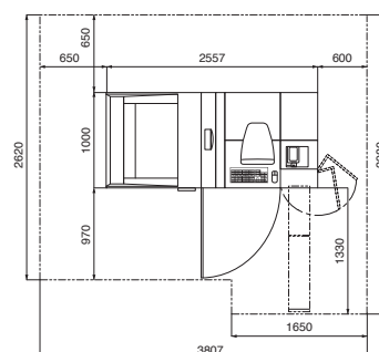
Space required for installation ( unit: mm )
